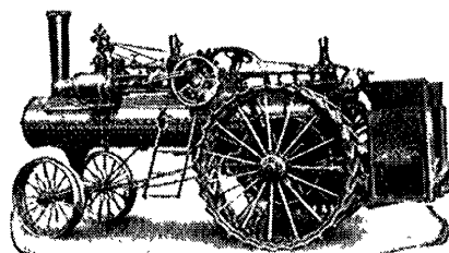
Longfellow High-Pressure Compound
